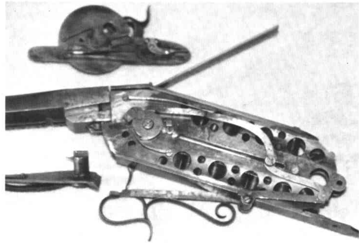
The trigger guard lever starts down, ramrod starts forward, nipple wheel arm slightly forward.
