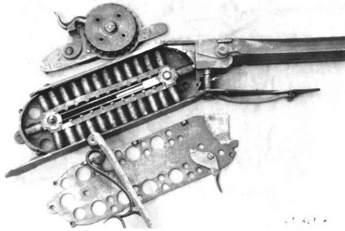
Now the ramrod has pushed a cartridge into the chamber. Note nipples on wheel above, trigger on plate below.
