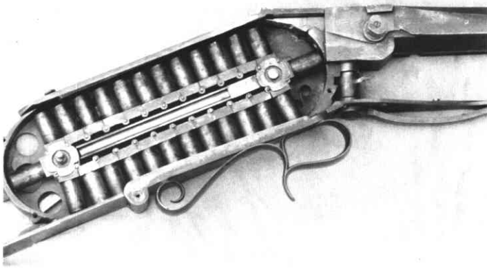
Right side of the action, lever closed, loading ramrod in rest position.
