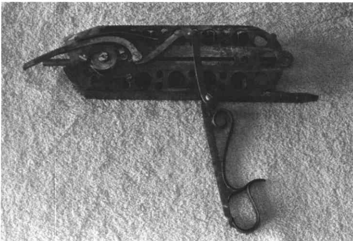
The action out of the frame: lever full down, ramrod and nipple wheel arm forward.
