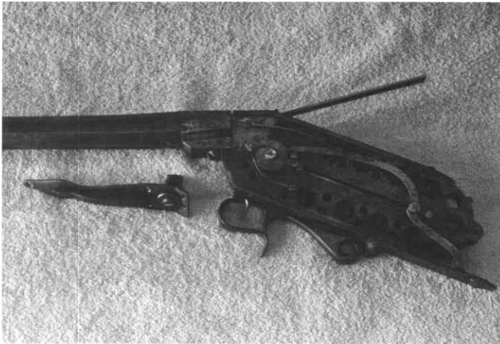
All at rest. The bottom of the swivel breechblock can be seen above and to the right of its lever.
