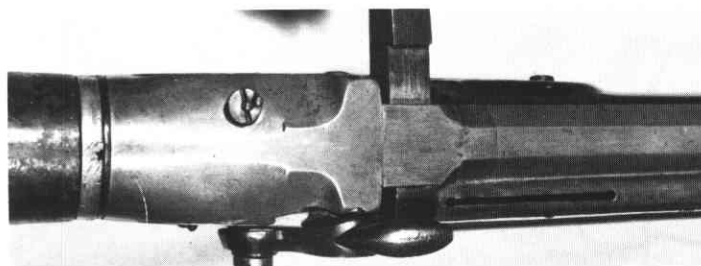
Fig. 2A: Same, showing end of magazine tube and loading bar of Girardoni system.
