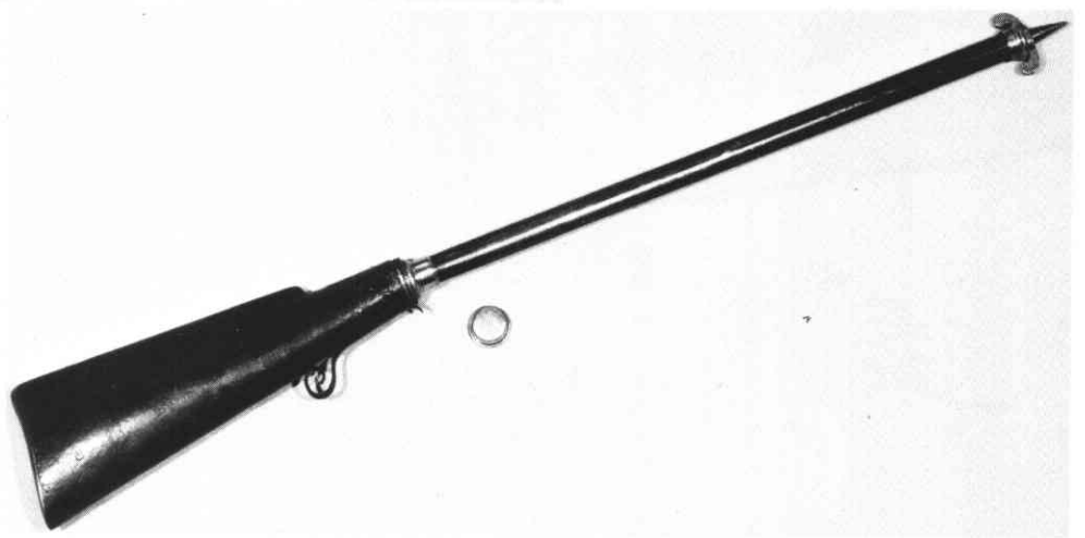
Fig. 7: Philadelphia butt reservoir attached to its pump ready to be screwed into shoulder-level point on tree for pump-up.
