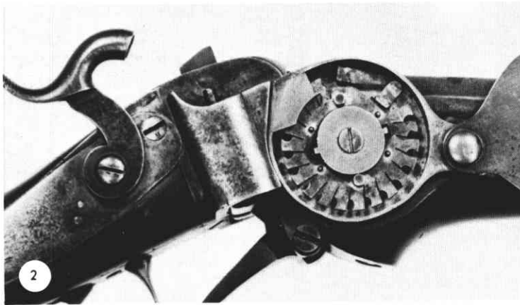
2nd model Sharps priming mechanism
