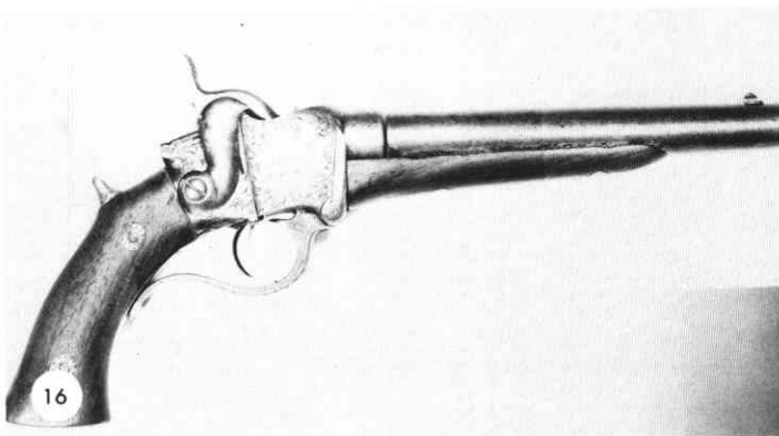
Hartford single shot pistol.
