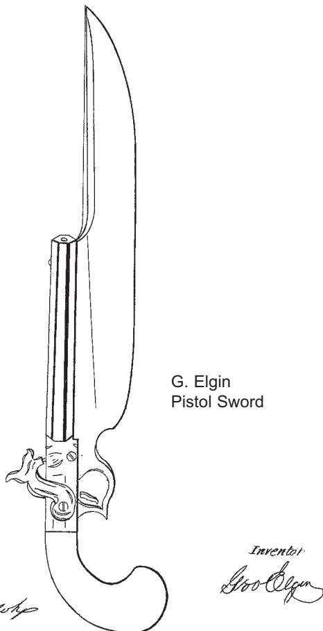
Figure 3. Patent drawing of George Elgin's bowie-knife cutlass pistol (U.S. Pat. # 254 issued July 5, 1837). Allen made the pistol and N.P. Ames provided the knife blades.
