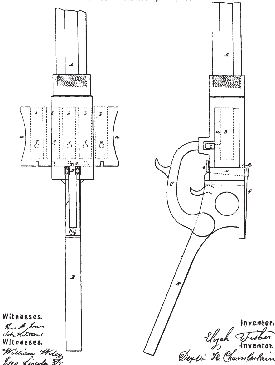
Figure 6. Patent drawing of Elijah Fisher and Dexter H. Chamberlain's "harmonica"-style magazine repeating rifle (U.S. Pat. # 168 issued April 17, 1837). The chamber block slides laterally through a mortise between barrel and breech. A vertically sliding wedge eliminates space between the mouth of a chamber and the breech of the barrel. Elijah Fisher was a Springfield resident.
