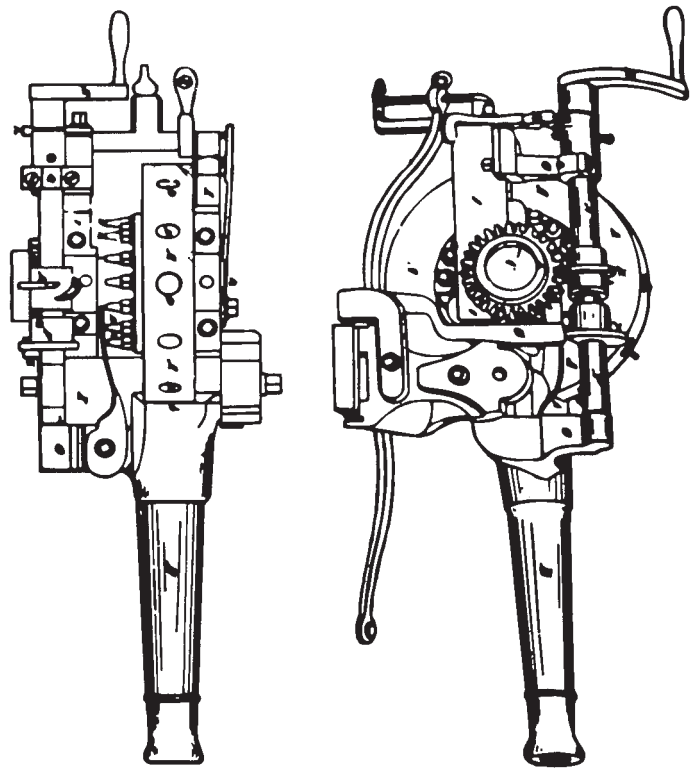
Figure 2. Patent drawing of John Webster Cochran's "rotary cannon" (U.S. unnumbered patent issued October 22, 1834). Allen made the mechanisms and N.P. Ames cast the bronze barrels. Cochran's rotary cannon is considered one of the earliest of Allen's special projects.
