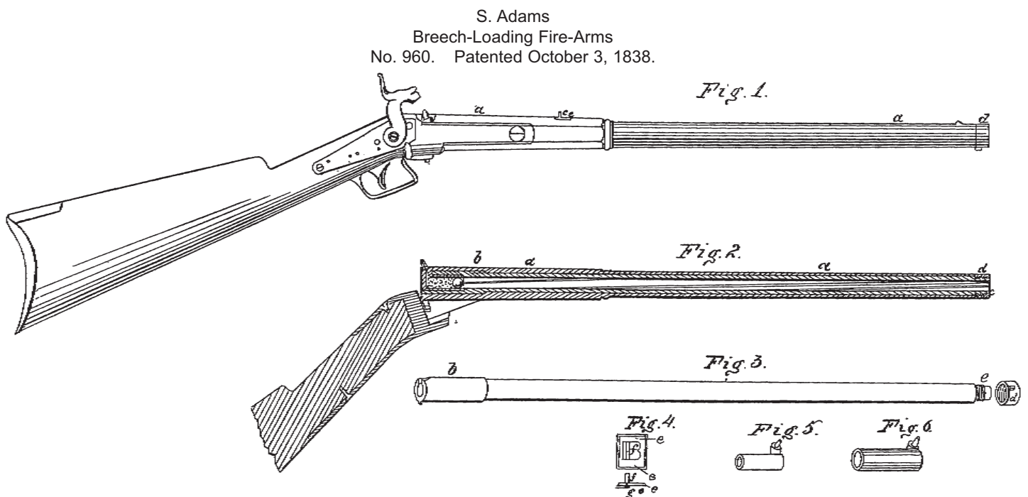
Figure 5. Patent drawing of Samuel Adams’ single-shot combination rifle/shotgun, utilizing a removable rifled barrel liner and steel auxiliary percussion chambers conforming to each mode of use (U.S. Pat. # 960 issued Oct. 3, 1838). The back-action locks were marked “C.B. Allen” and the barrels were engraved “Samuel Adams Patent” in script and stamped “Chicopee Falls Co. Mass.” Adams was a Springfield resident.
